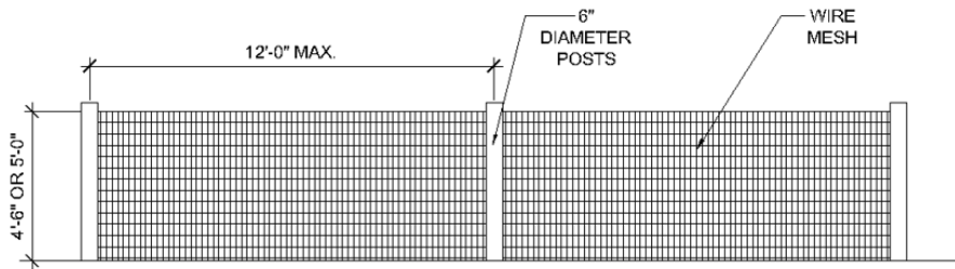
FENCE ELEVATION (FENCE OPTION 3) NOT TO SCALE
