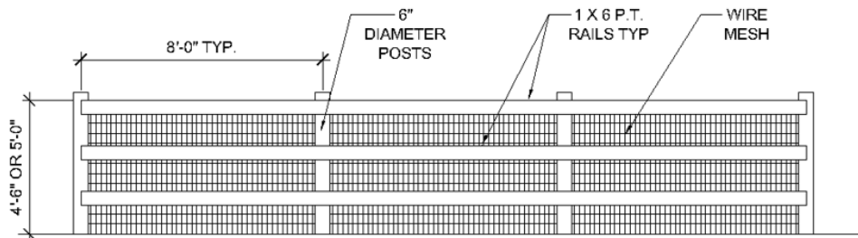
FENCE ELEVATION (FENCE OPTION 2) NOT TO SCALE
