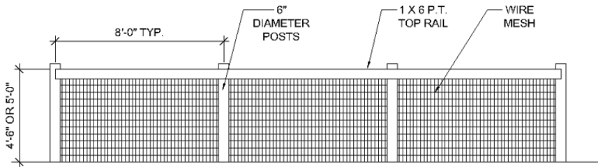
FENCE ELEVATION (FENCE OPTION 1) NOT TO SCALE
